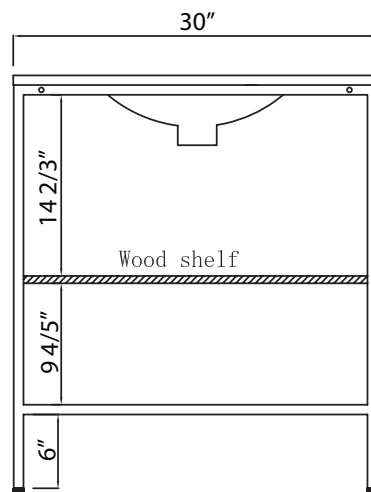
BACK VIEW
