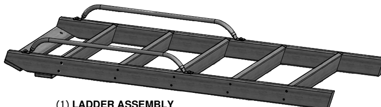
(1) LADDER ASSEMBLY
