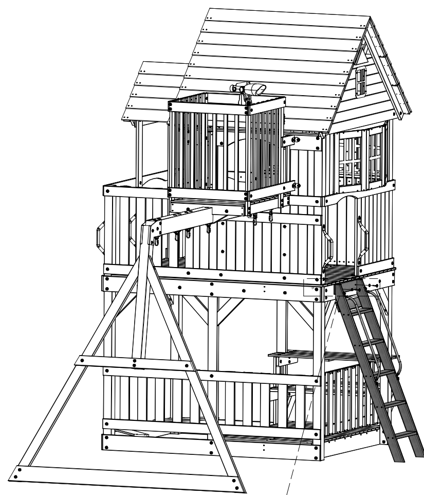
(1) LADDER ASSEMBLY
