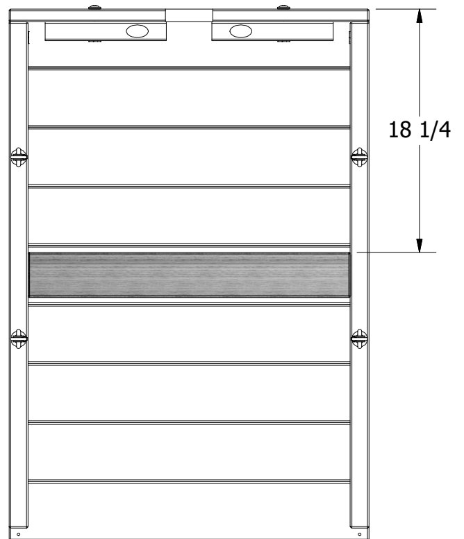
BOTTOM VIEW
