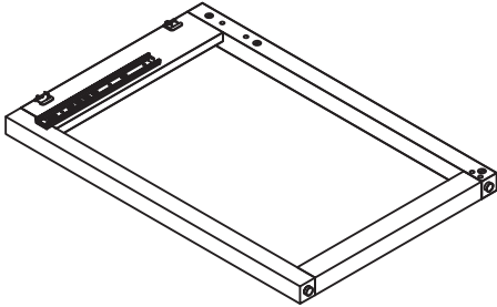
(C) Left Leg Frame (1 PC)
