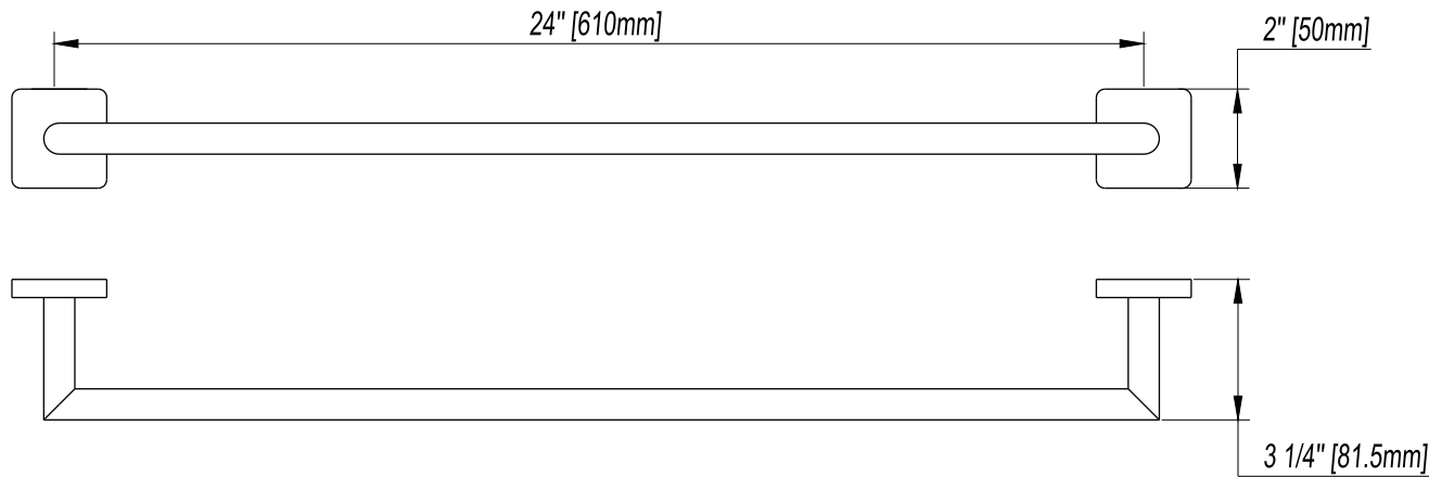
SINGLE TOWEL BAR / BARRA DE TOALLA SIMPLE / BARRE PORTE-SERVIETTES SIMPLE
