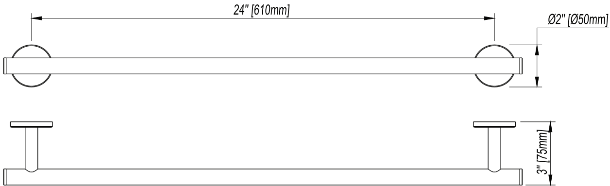
SINGLE TOWEL BAR / BARRA DE TOALLA SIMPLE / BARRE PORTE-SERVETTES SIMPLE
