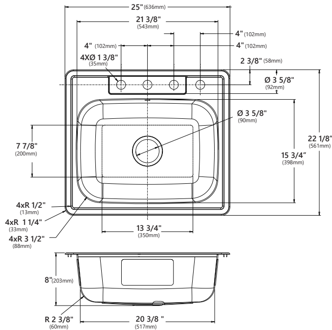
Model #: KTM101-25 Sink Dimensions: 25" x 22" x 8" Min Cabinet Size: 28" Strainer: ST-1
