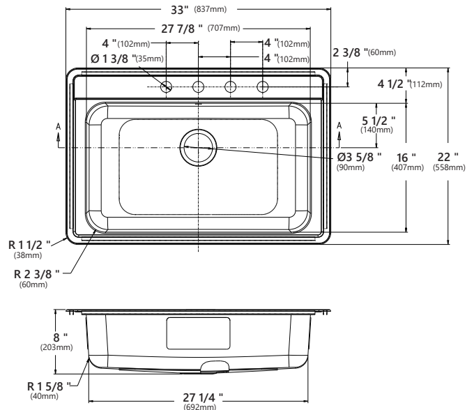
Model #: KTM100-33 Sink Dimensions: 33" x 22" x 8" Min Cabinet Size: 36" Strainer: ST-1
