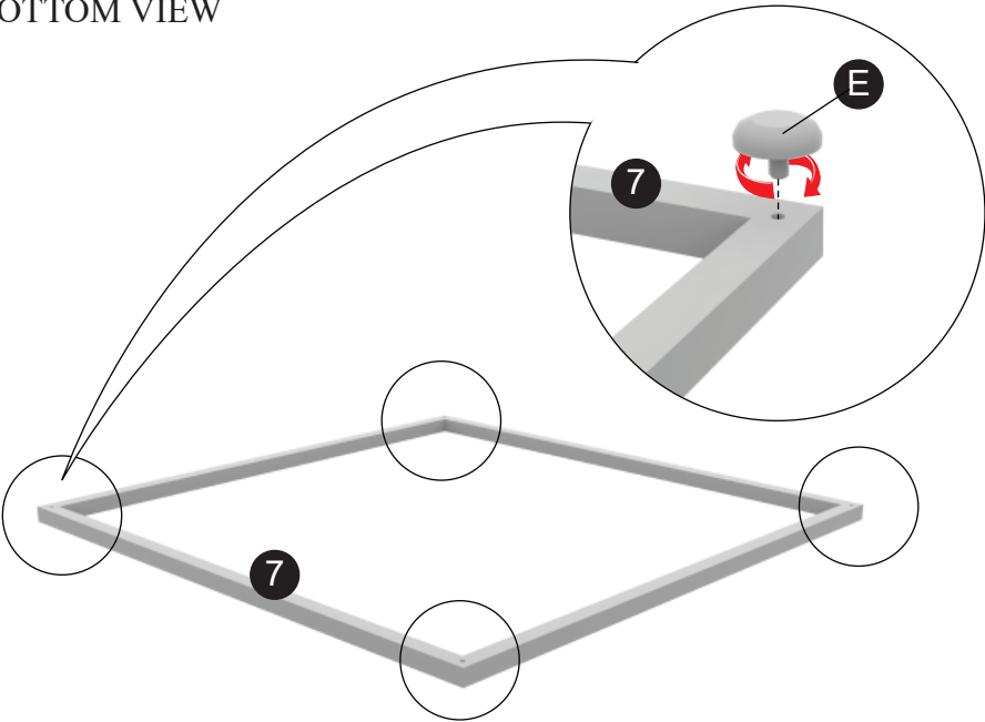
STEP 6 BOTTOM VIEW
