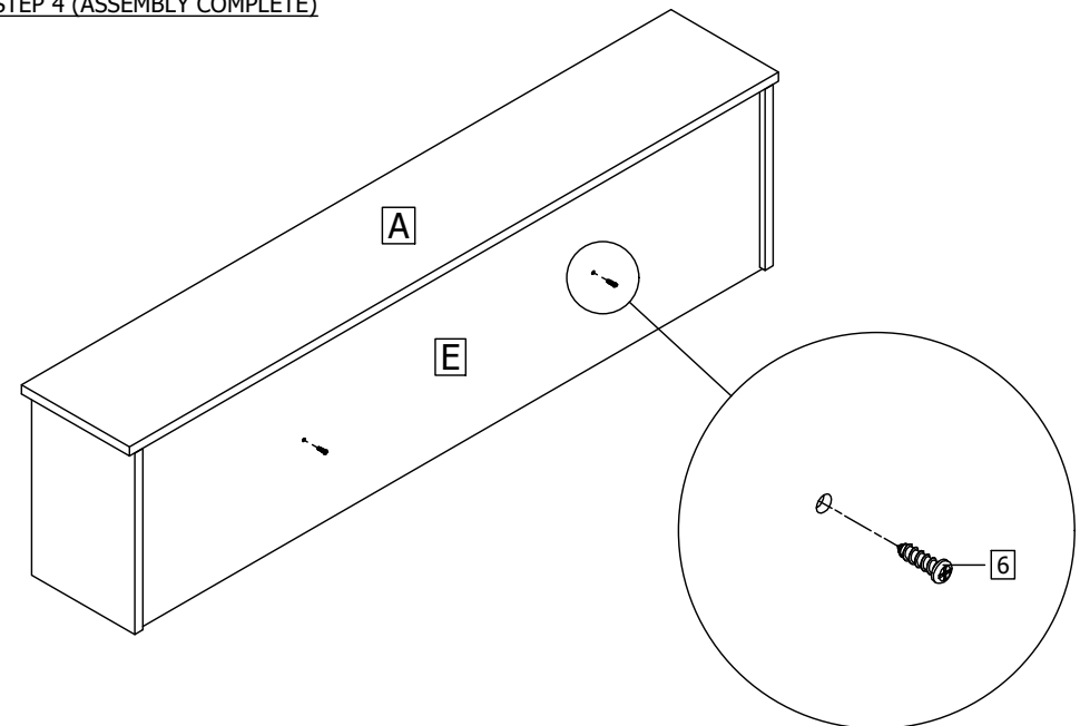
STEP 4 (ASSEMBLY COMPLETE)
