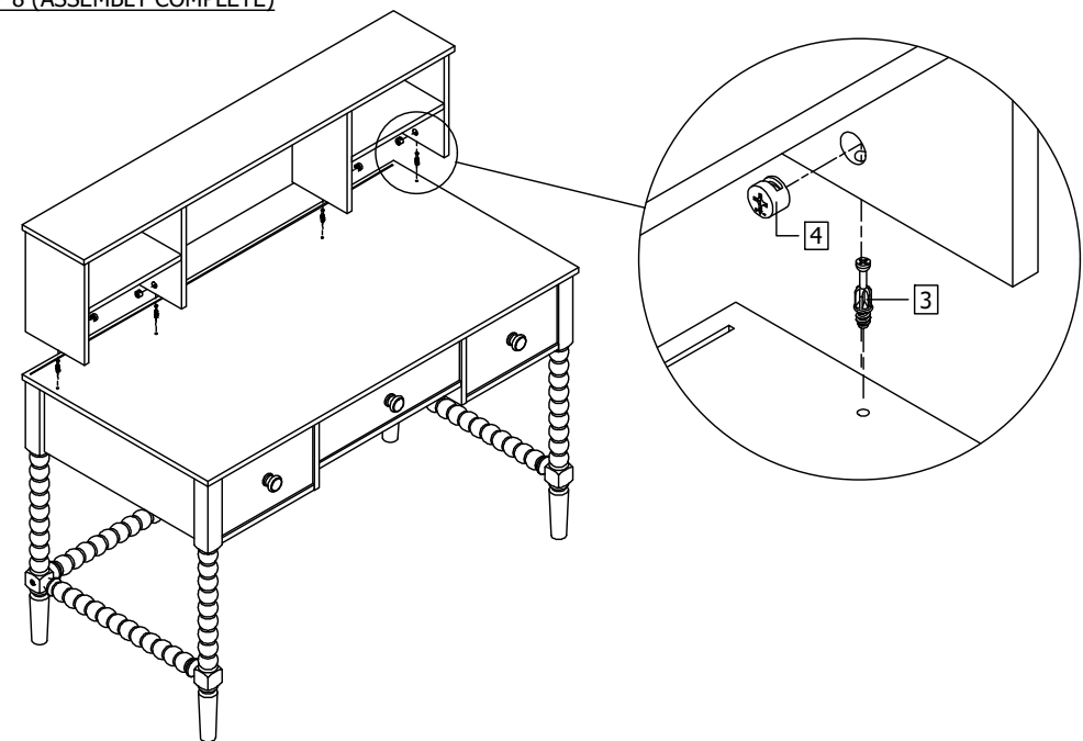
STEP 8 (ASSEMBLY COMPLETE)
