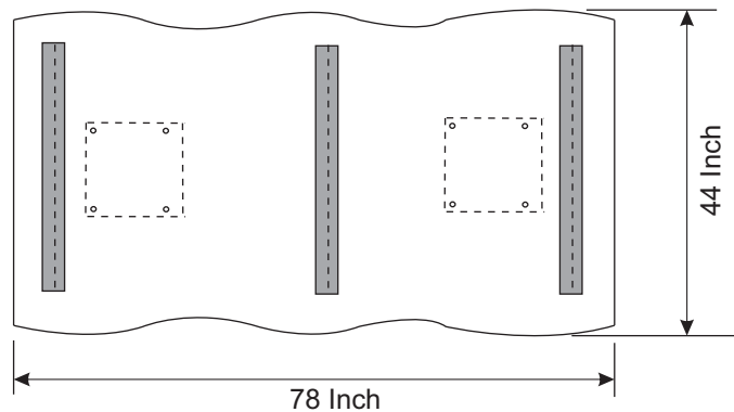
TOP BOTTOM VIEW
