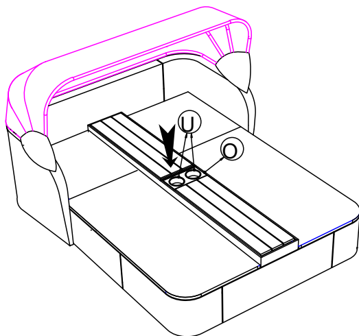
STEP 25 : Connect the part from step 24, Metal Tray (O), PlasticTray (U).
