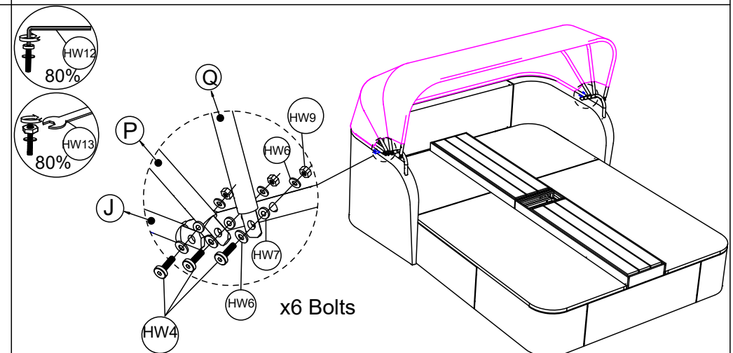
STEP 20: Connect the part from step 14, step 19, tighten Bolt (HW4), Flat Washer (HW6), Washer M6x5mm (HW7), Nut M6 (HW9) with Allen Key (HW12), Key (HW13).
