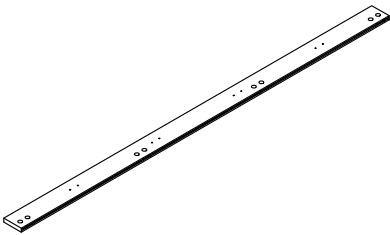
⑫ 1583.5*75*15= 2PCS
