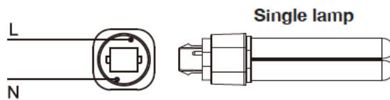
Wiring Diagram 1: New Fixture Without Ballast
