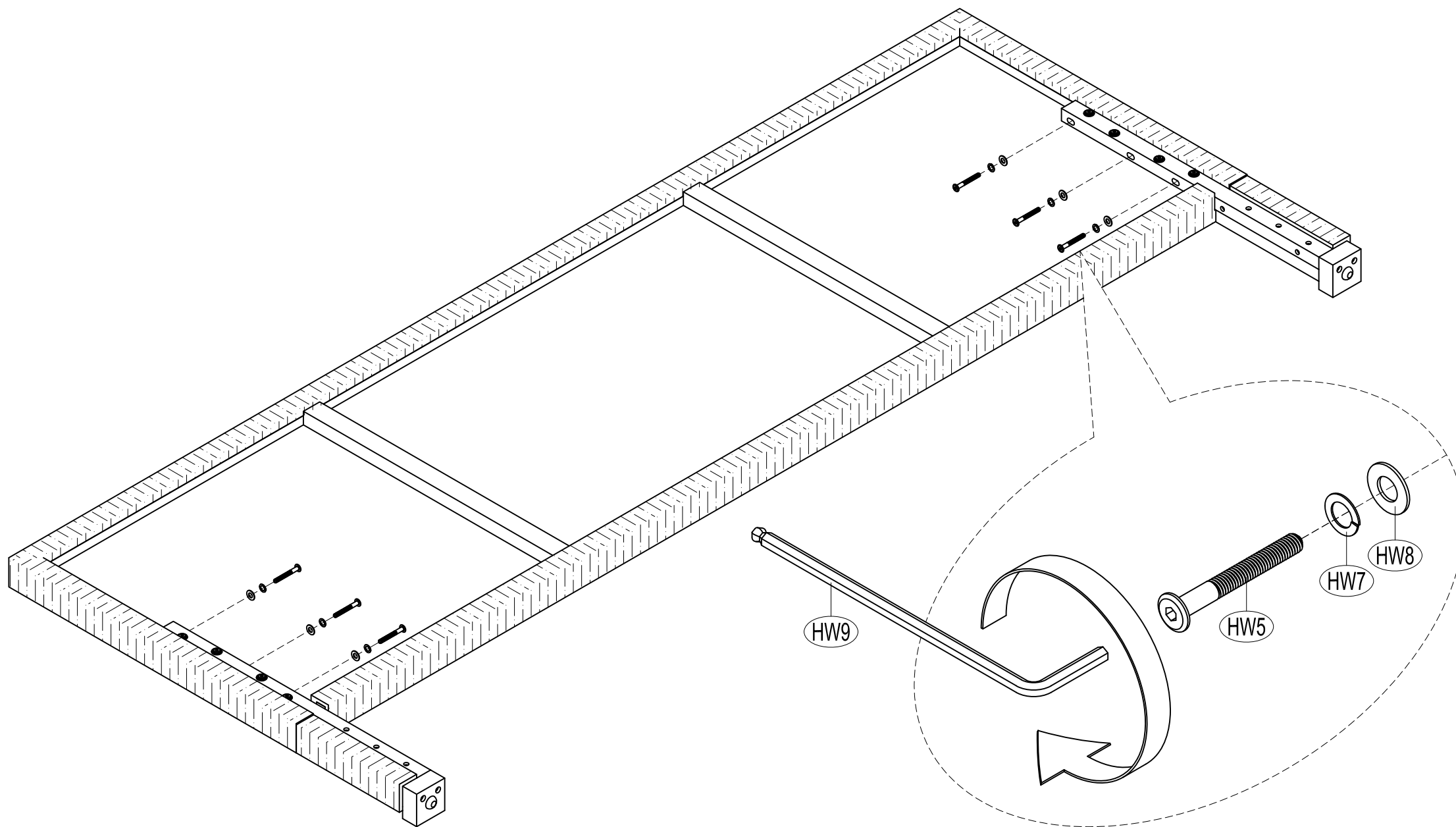
STEP 2 ATTACH BOLTS 50 MM (HW5), SPRING WASHERS (HW7) AND FLAT WASHERS (HW8) TO UNIT. TIGHTEN BOLTS USING L KEY (HW9).
