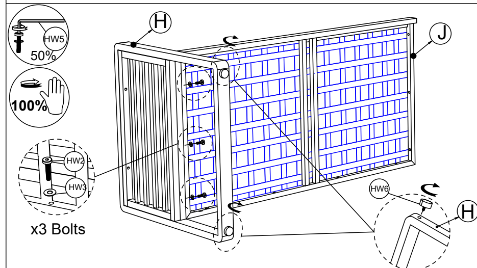
STEP 7: Tighten Adjustable Feet (HW6). Connect Left Armrest (H), Bench-2 Seat (J), tighten Bolt (HW2), Flat Washer (HW3) with Allen Key (HW5).
