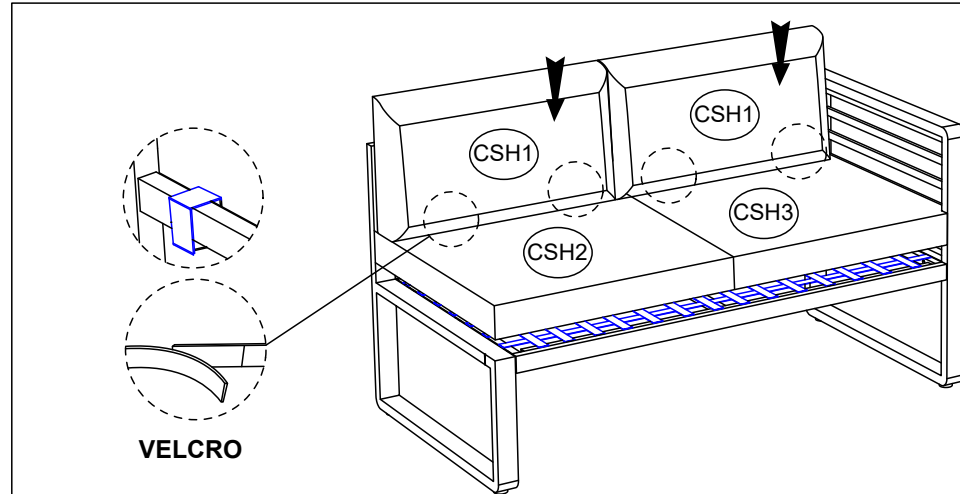
STEP 5 : Set up Cushion (CSH1), (CSH2), (CSH3)
