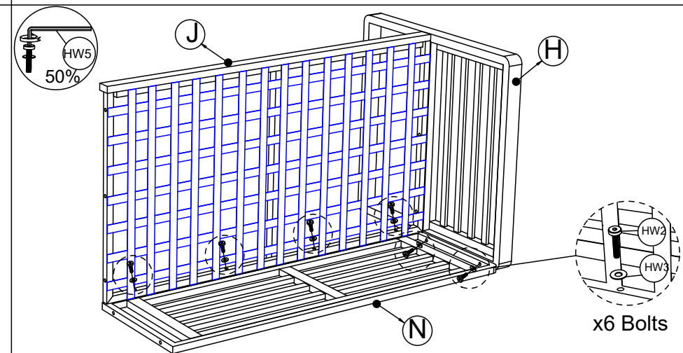
STEP 8: Connect part from step 7 & Left Bench-2 Back (N), tighten Bolt (HW2), Flat Washer (HW3) with Allen Key (HW5).
