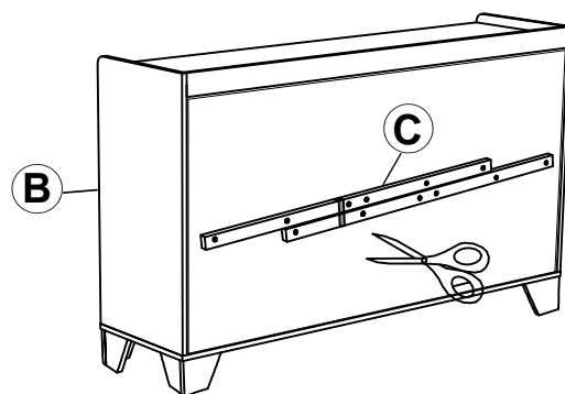
**BACK VIEW**
