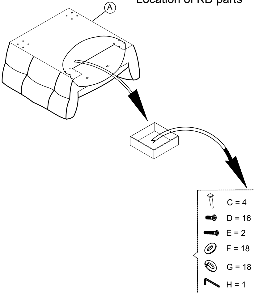
Location of KD parts
