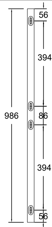
Back Rail
