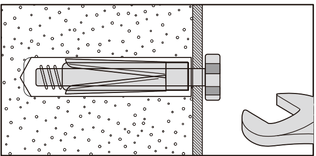
No.6 "Shield Anchor" wall plug - heavy loads
