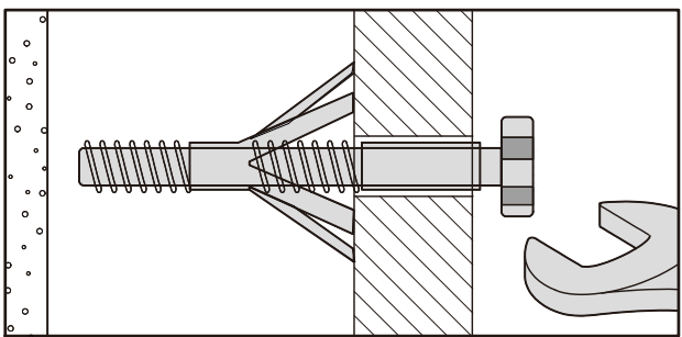
No.4 "Cavity Fixing - Heavy Duty" wall plug
