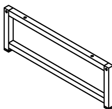
SIDE METAL FRAME 17.68" X 5.9" X 0.75" 2PCS
