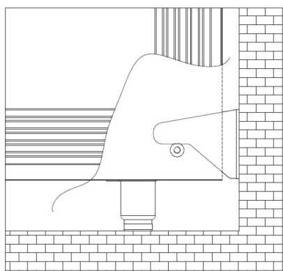
Anti-tip device for XGR24403
