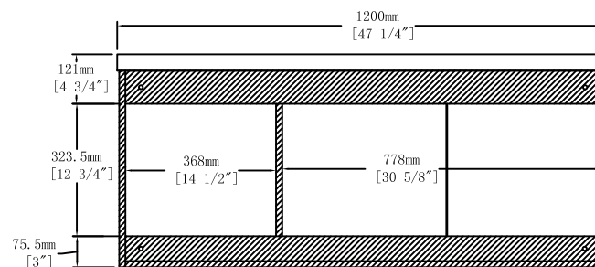
Back View
