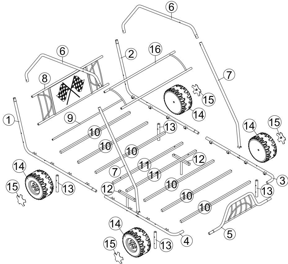
Exploded View
