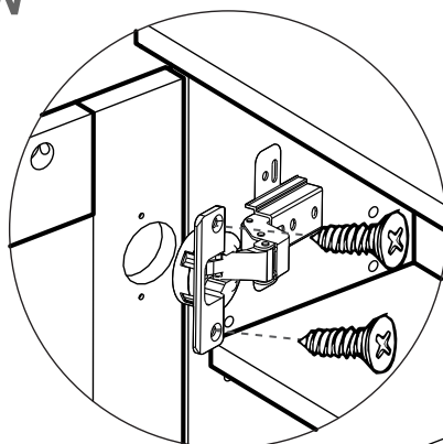
HEIGHT ADJUSTMENT
