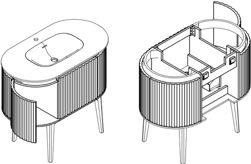
Perspective View
