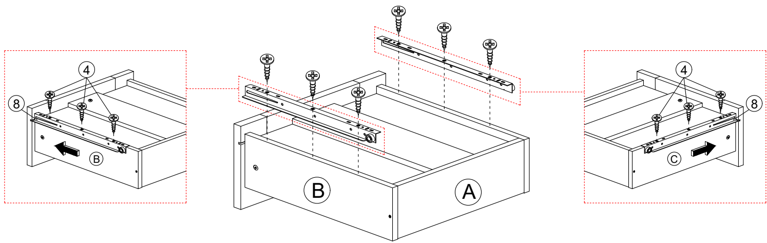
Bottom View
