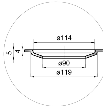
Detail 1 – Drain (1:2.5)
