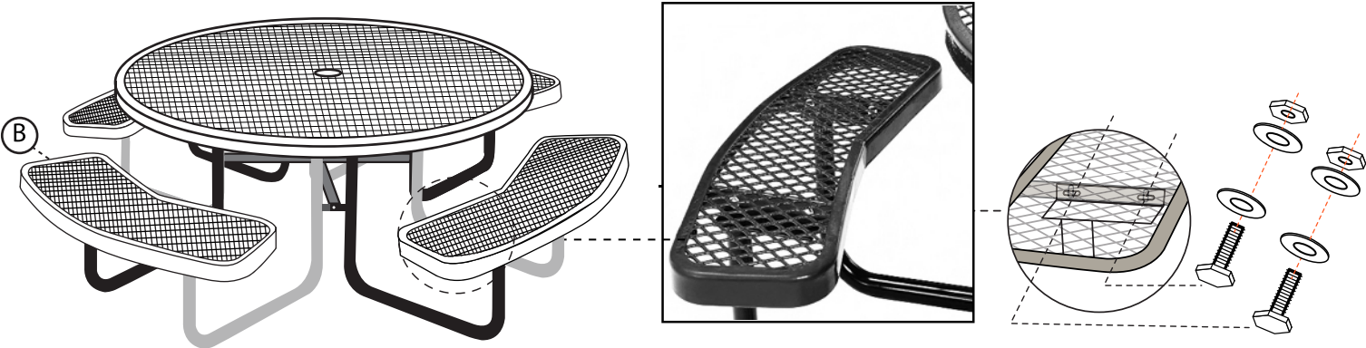
Step 3 Assembly of the Legs and Seats
