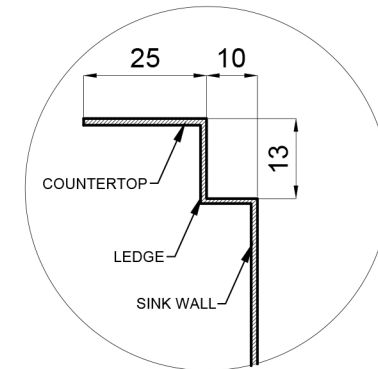
Detail 1 – Inner ledge(mm) (1:2.5)
