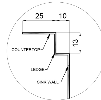
Detail 1 – Inner ledge(mm) (1:2.5)
