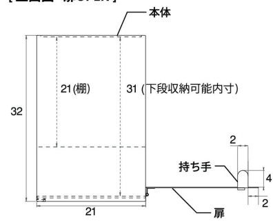
[上面図・扉OPEN]
