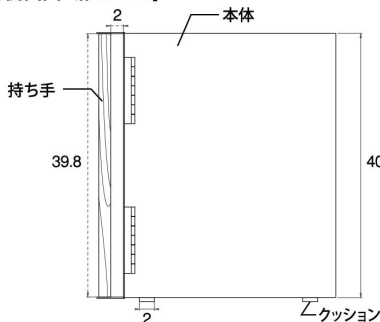
[側面図・扉CLOSE]
