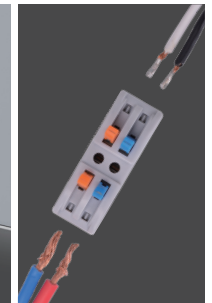
2. Through the connector provided, here is how: a. remove the plug by pull up the buttons of the connector b. connect the wire from your home power source to one end of the connect c. make sure all wires settled firmly
