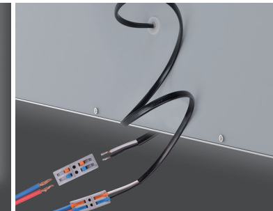
2. Through the connector provided, here is how: a. remove the plug by pull up the buttons of the connector b. connect the wire from your home power source to one end of the connect c. make sure all wires settled firmly
