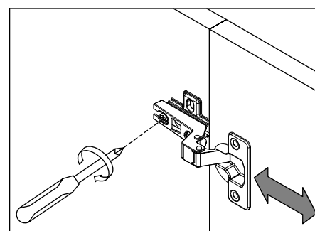
C. Front-to-Back by the slacking the hinge arm mounting screw
