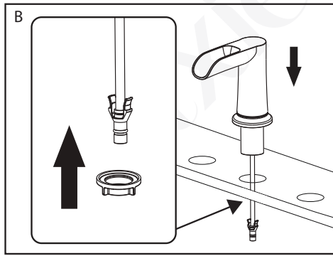
B. Place spout through the center mounting hole on the countertop. Secure spout with the locking nut.
