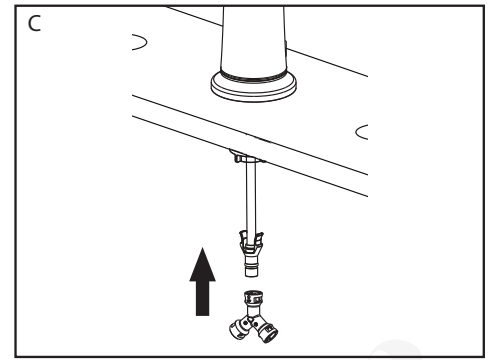
C. Insert the Tee connector to the center spout inlet hose until it clicks in place. Make sure the hose is fully inserted. There will be an audible click when the connector is connected properly.
