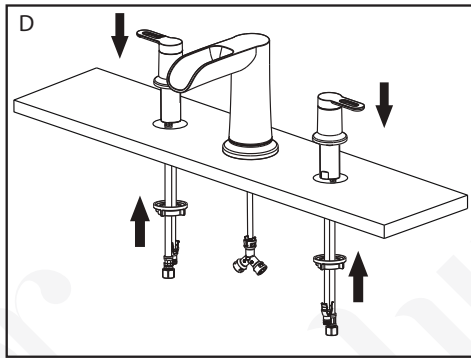
D. Place hot and cold water handles through the 2 mounting holes. Handles should point outward in off position. Secure the handles with locking nuts.
