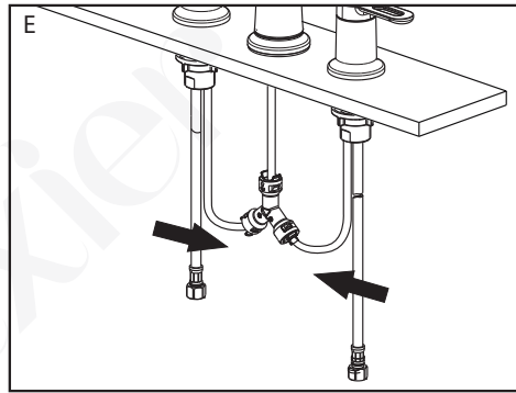
E. Connect the 2 supply hoses to the Tee connector. Make sure the hose are fully inserted until locked in place. There will be an audible click when the hoses are connected properly.
