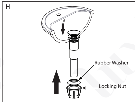
H. Remove rubber washer and locking nut from the drain assembly and slide the drain into the sink. Install the rubber washer first and tighten the locking nut to install the drain. Connect the drain to the P-trap and waste pipe.
