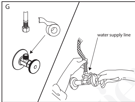
G. Apply Teflon (PTFE) tape on the shut off valves. Thread the tape in counter-clockwise direction. Use an adjustable wrench to tighten the hoses. (IMPORTANT: Do not overtighten the connections.)
