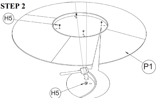
COMPLETE ASSEMBLY
