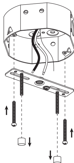
Mounting Screws
