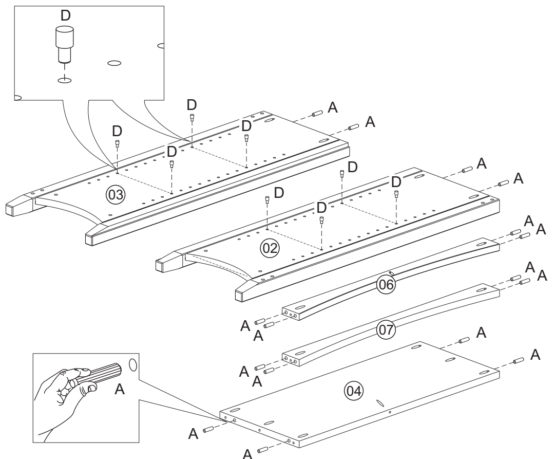
A - 8,0x30 Wood Dowel Qty. 16
