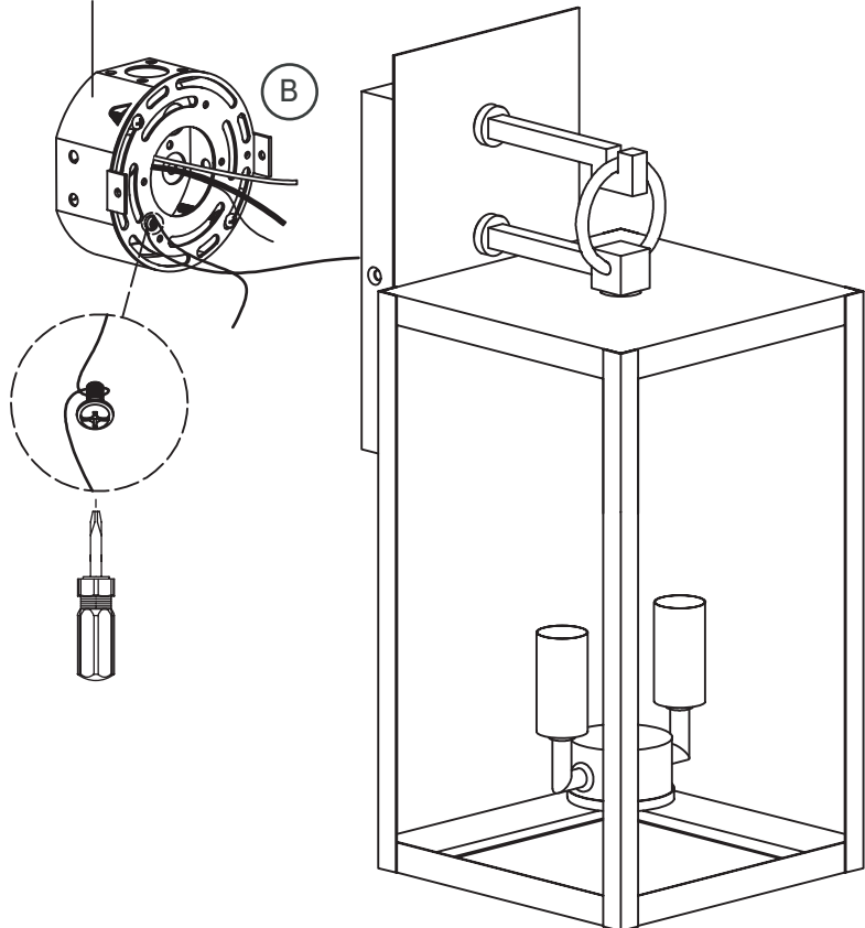
Electrical box
