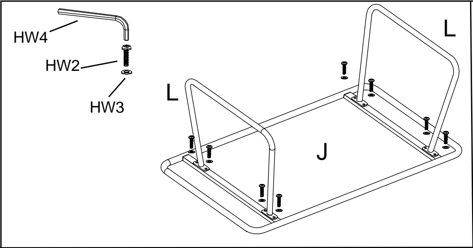
STEP7: Assemble the table leg (L) to the table top(J),using bolt. washer(HW3&HW2) and Allen key(HW4)
