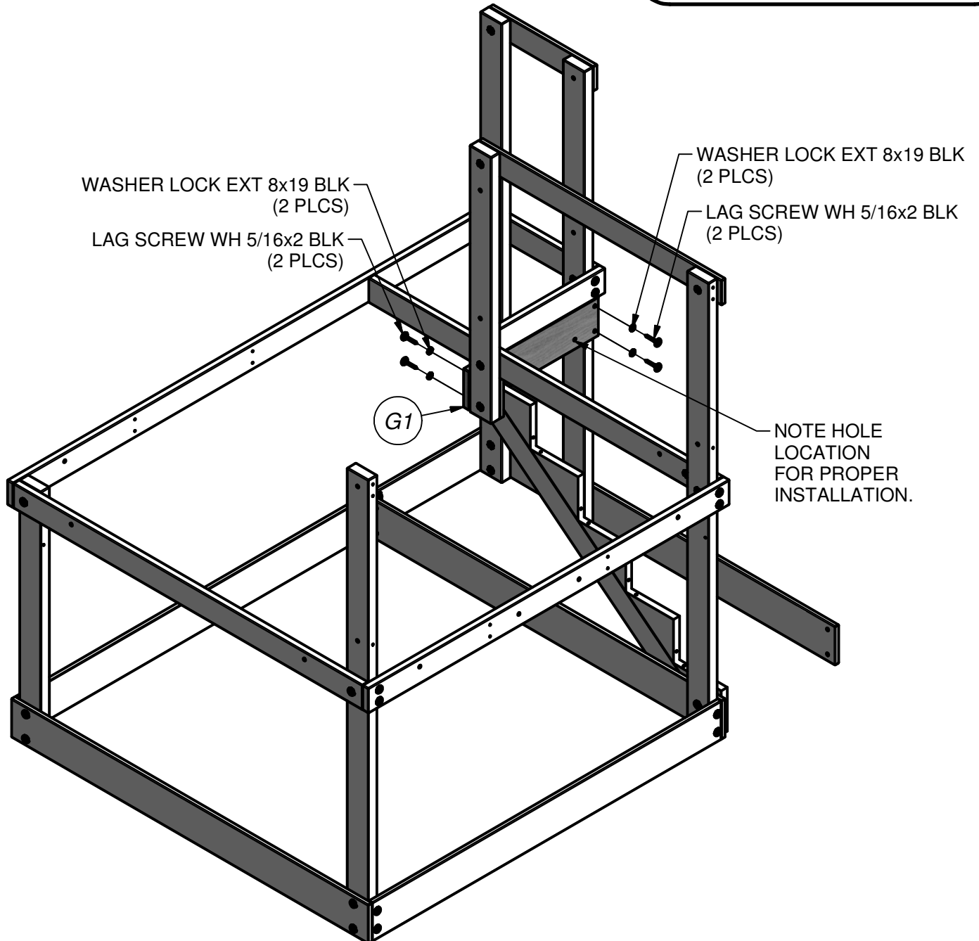
(4) LAG SCREW WH 5/16x2 BLK
