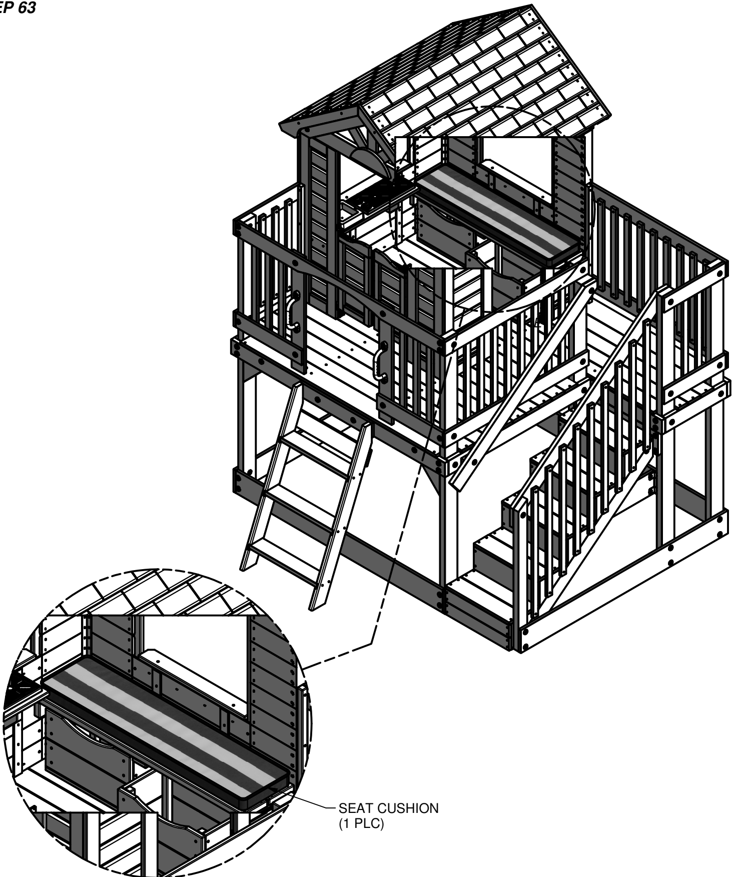
(1) - SEAT CUSHION - A6P00107
