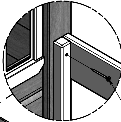
(1) PLAYHOUSE ASSEMBLY
