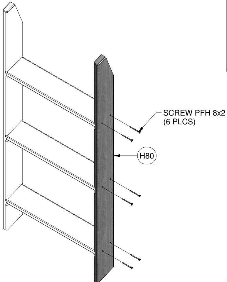
(6) SCREW PFH 8x2
