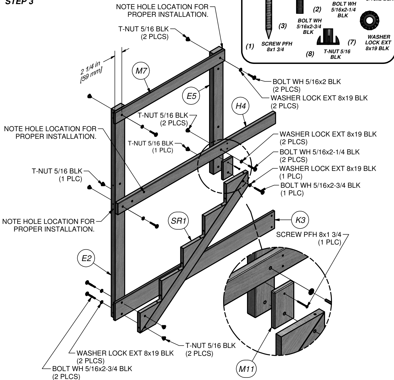
(1) M7 - WALL RAIL - W4L06643 5/8"x3 3/8"x38 1/4" (16x86x970)
