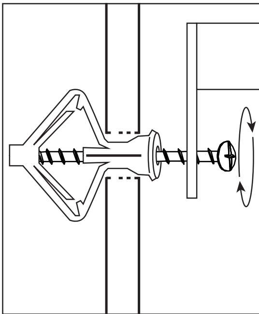
3. Begin tightening
