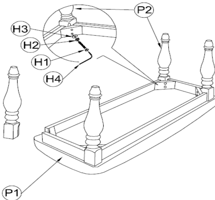
COMPLETE ASSEMBLY
