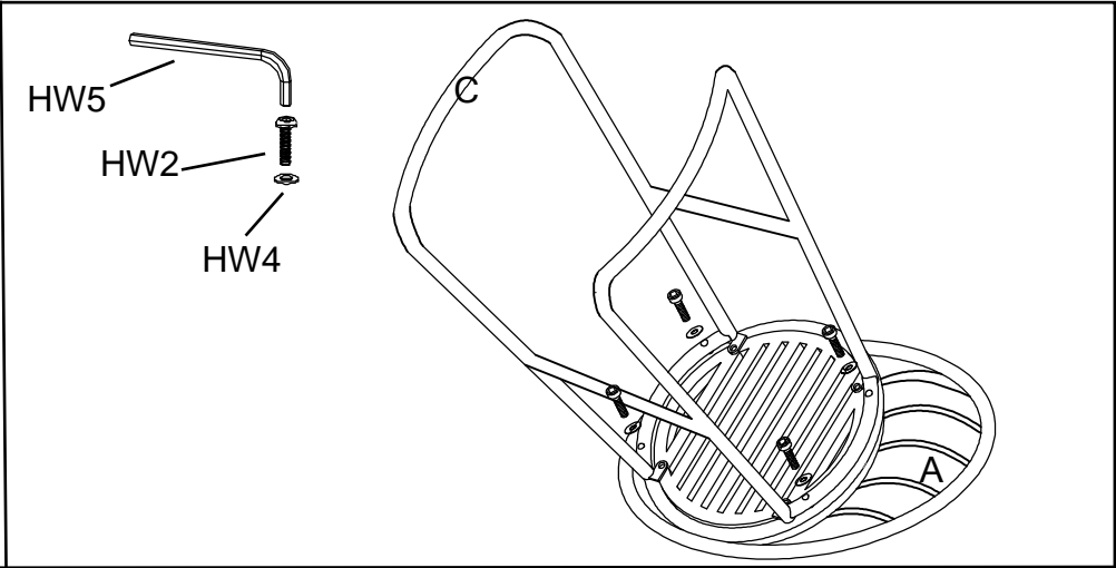
STEP5: Assemble the chair leg(C) to the chair(A). using bolt and washer(HW2&HW4) and Allen key(HW5)
