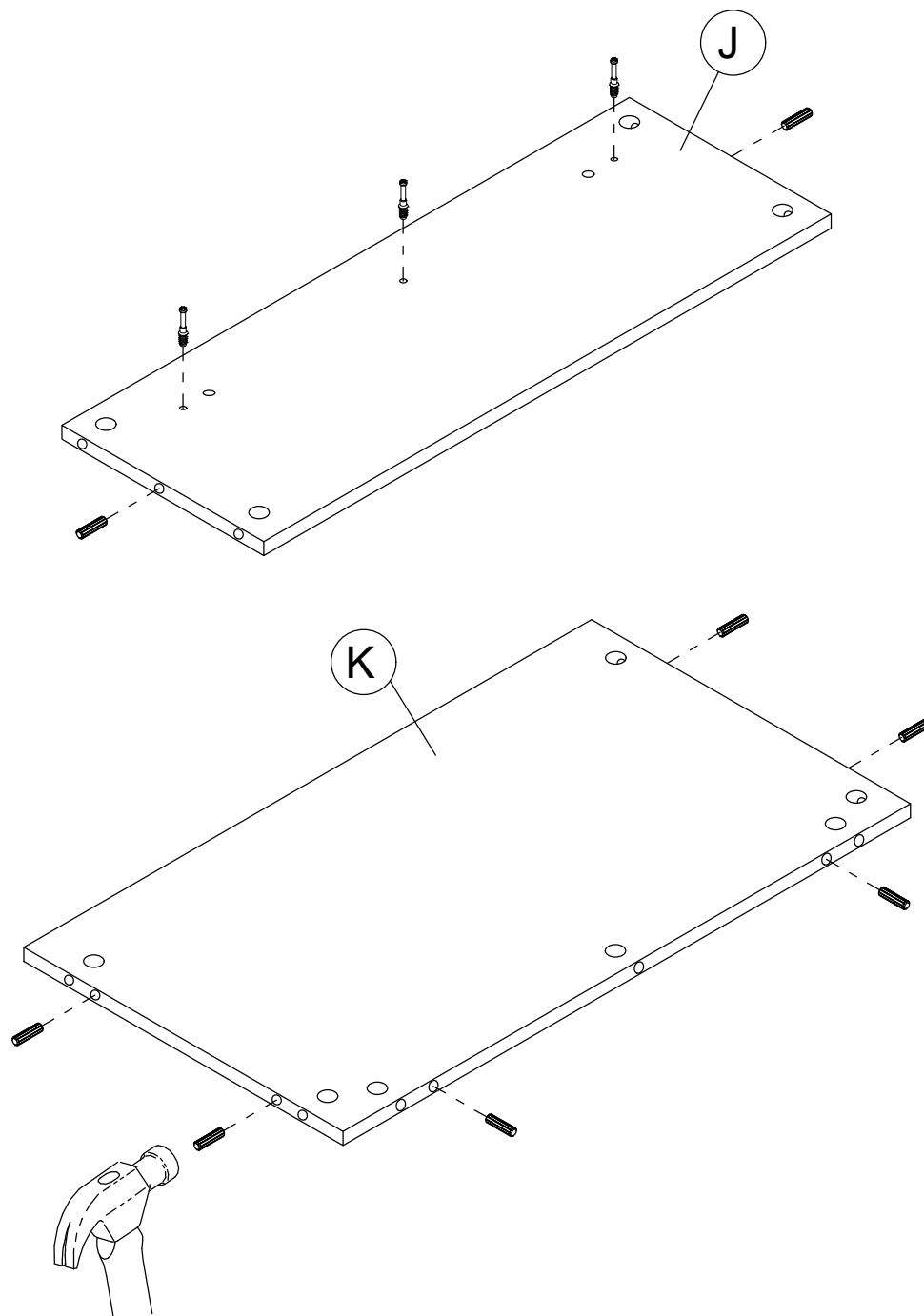
KD Bolt
