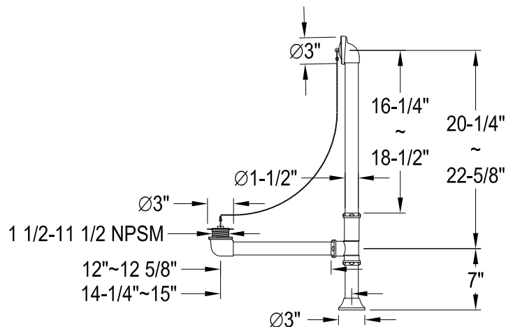
CC2091,2,5,7,8 Tub Waste & Overflow
