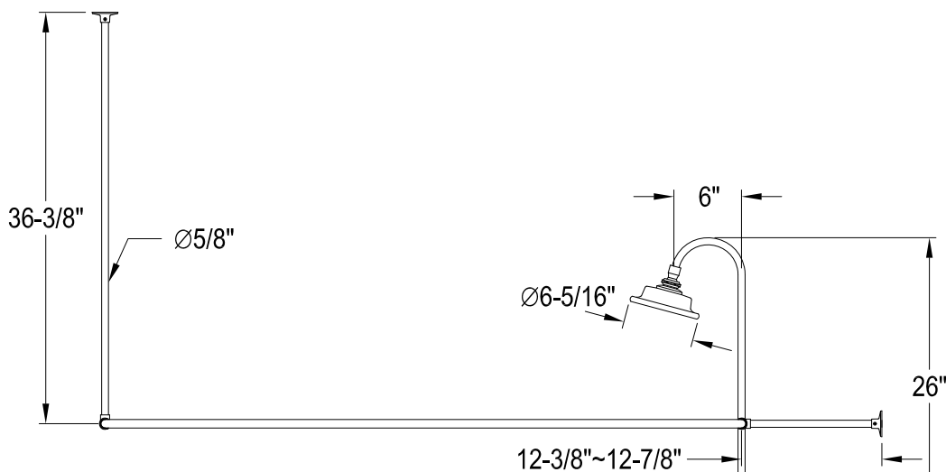
CC471,2,5,7,8 Double Offset Bath Supply
