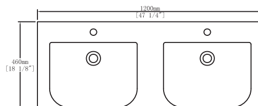
Top View (48D)
