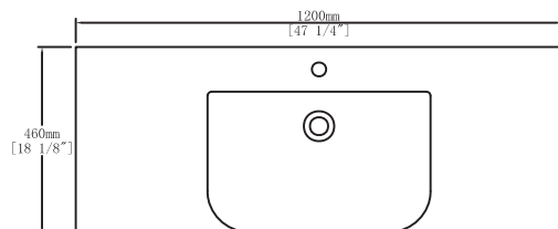
Top View (48S)
