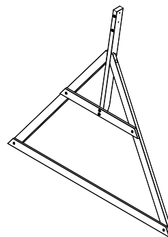
(1) SWING BEAM END SUBASSEMBLY
