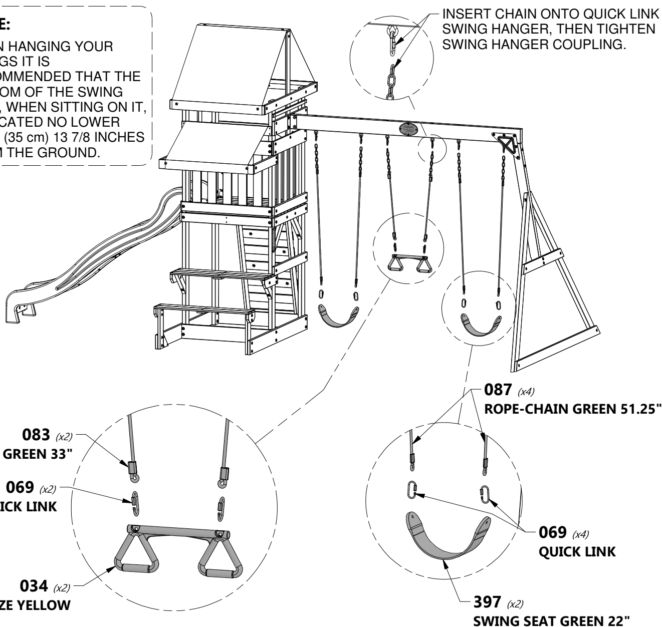
A100087 (4) | ROPE-CHAIN GREEN 51.25"
