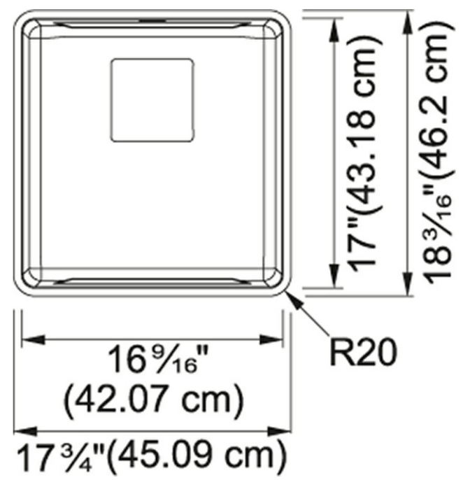
Technical Drawing
