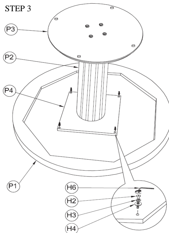
COMPLETE ASSEMBLY
