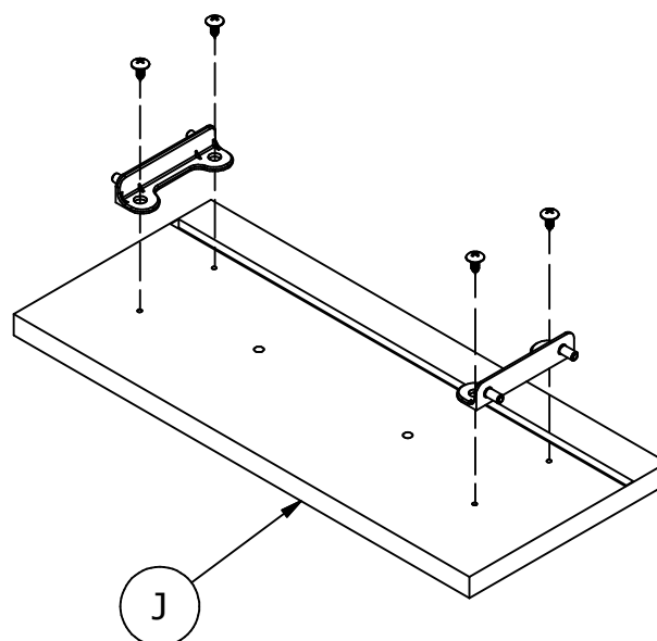
DWR Bracket
