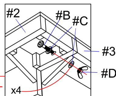
BOTTOM VIEW OF FOOTBOARD
